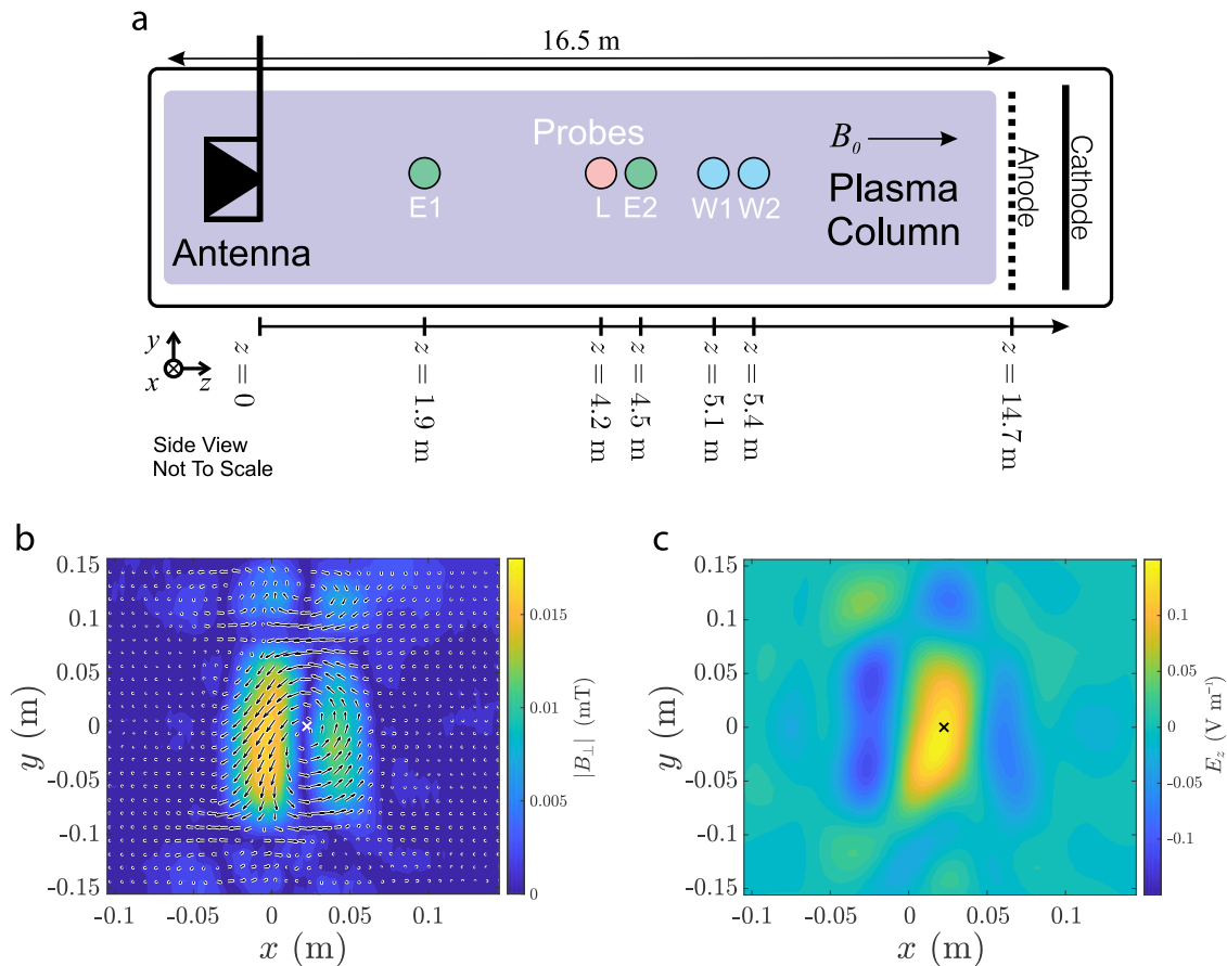
Fig. 1 LAPD setup and snapshots of the Alfvén wave. a Experimental setup showing the Sigma antenna, Elsässer probes (E1, E2), Langmuir probe (L), and WWAD probes (W1, W2). b Contour plot of B_{\perp}(x, y) of the inertial Alfvén wave in the plane perpendicular to B_0 measured at E2. Arrows indicate the magnitude and direction of B_{\perp}(x, y) . c The calculated E_z(x, y) midway between the WWAD probes W1 and W2. The x indicates the (x, y) location of the WWAD measurements of g_e(v_z) .
